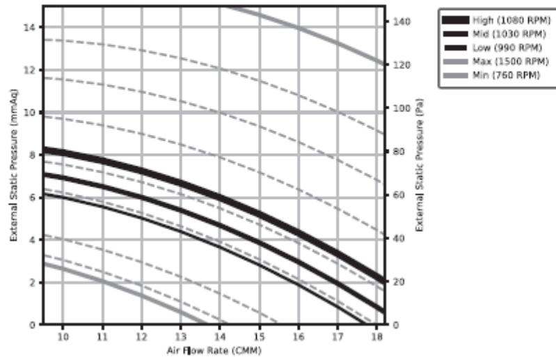
P-Q Curve
